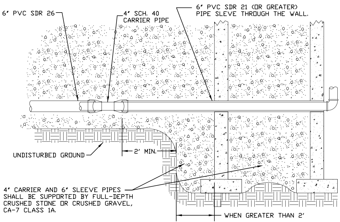
TYPICAL DETAIL FOR SANITARY SERVICE THRU PORCH BOX WALL
